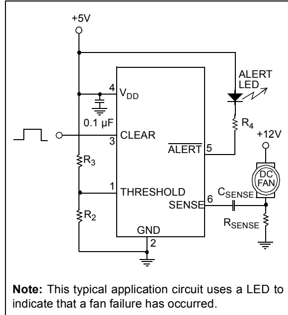
FIGURE 4-2: Typical Application Circuit.
