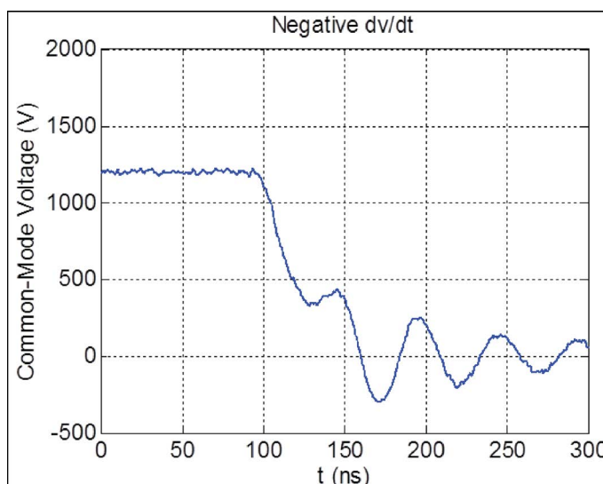
Figure 11. Applied Common Mode Pulses for Generating Negative dv/dt.
