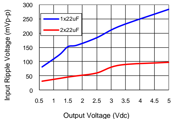
Figure 40. Input ripple voltage for various output voltages with 1x22 µF or 2x22 µF ceramic capacitors at the input (40A load). Input voltage is 12V.
