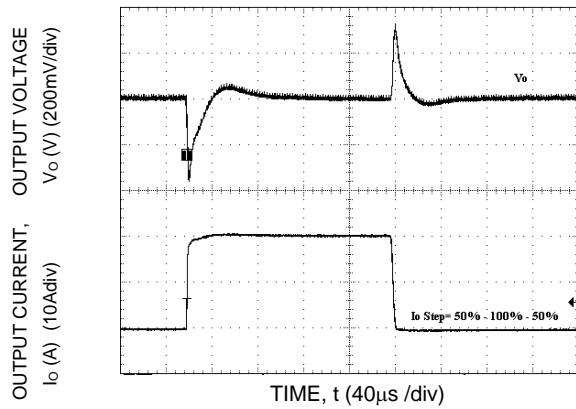
Figure 34. Transient Response to Dynamic Load Change from 0% to 50% to 100% to 50% with V_{IN}=12V .
