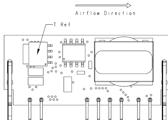
Figure 53. Temperature measurement location T_{ref} .
