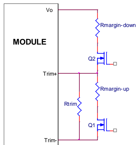
Figure 50. Circuit Configuration for margining Output voltage.
