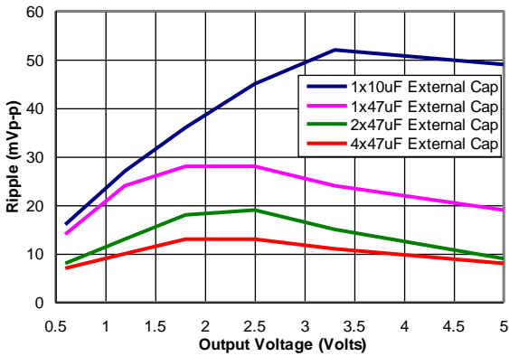
Figure 47. Output ripple voltage for various output voltages with external 1x10 μF, 1x47 μF, 2x47 μF or 4x47 μF ceramic capacitors at the output (10A load). Input voltage is 12V.
