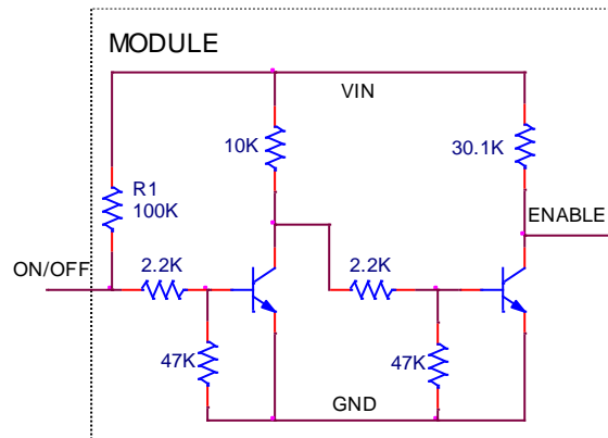
Figure 48. Remote On/Off Implementation.
