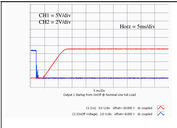
Vo=18V Typical startup characteristic from on/off at full load. Ch1 - output voltage, Ch2 – on/off signal
