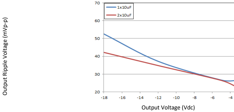
Figure 68. Output ripple with 1x10µF or 2x10µF output ceramic capacitors (max load).
