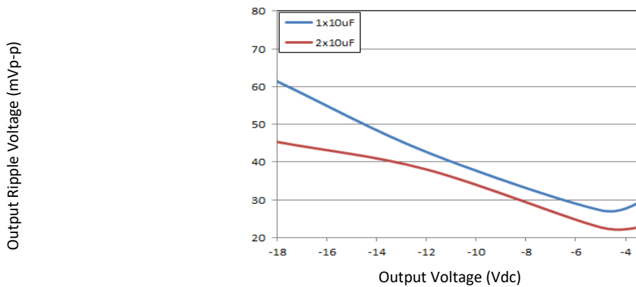
Figure 69. Output ripple with 1x10µF or 2x10µF output ceramic capacitors (max load).
