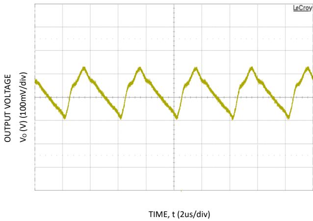
Figure 3. Typical output ripple and noise ( C_o=66 \mu F ceramic, V_{in} = 12V , I_o = I_{o,max} ).
