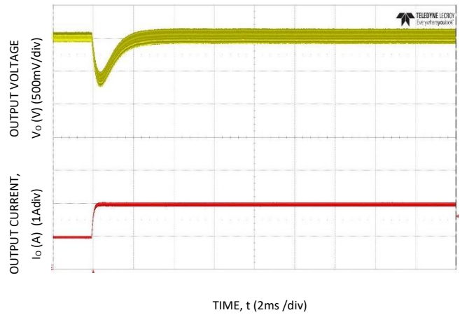
Figure 4. Transient Response to Dynamic Load Change from 50% to 100% at 12Vin, C_{out}=12 \times 4.7 \mu F , C_{Tune}=820 pF , R_{Tune}=30.1 k
