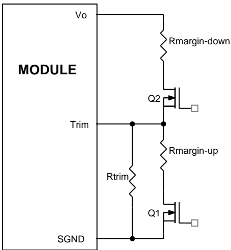
Figure 31. Circuit Configuration for margining Output voltage.
