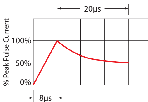
Figure 4. 8/20 \mu s waveform
