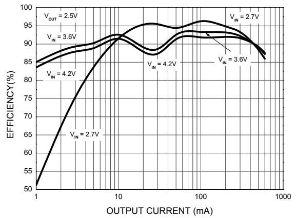
Fig. 6 Efficiency vs. Output Current
