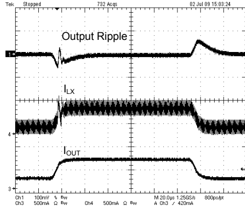
Fig. 15 Load Transient Response
