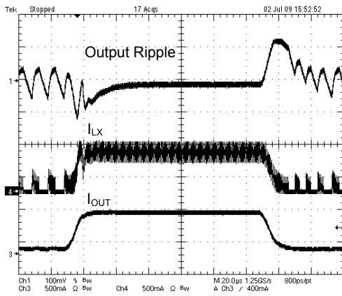
Fig. 16 Load Transient Response
