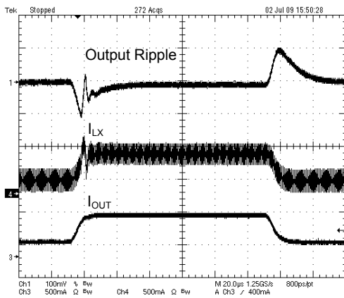
Fig. 18 Load Transient Response
