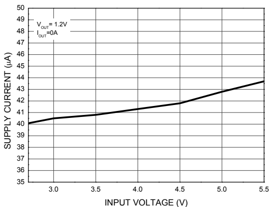
Fig. 12 Supply Current vs. Input Voltage
