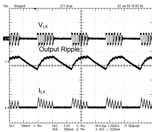
Fig. 19 PFM Operation
