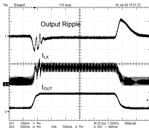
Fig. 17 Load Transient Response
