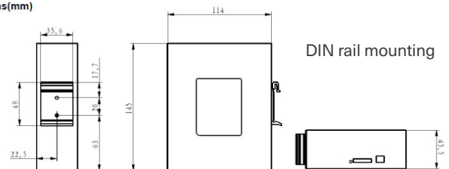
Dimensions(mm)
