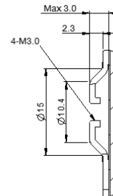
SECTION C-C SCALE 2/1
