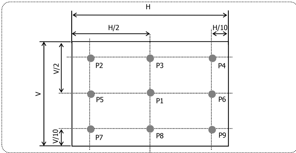
FIG.8 Measure Point for Luminance
