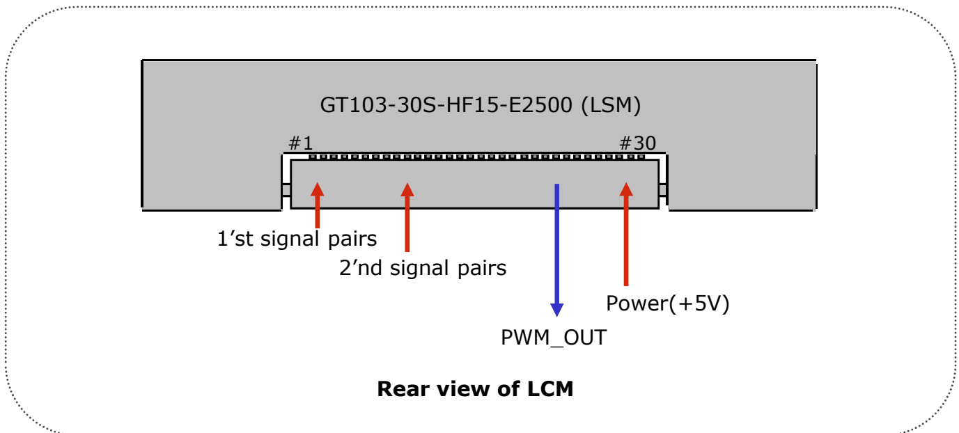
FIG. 4 Connector diagram
