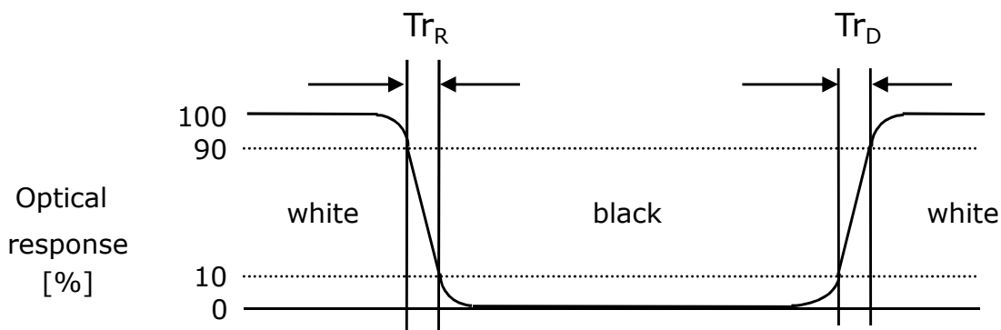
FIG. 9 Response time
