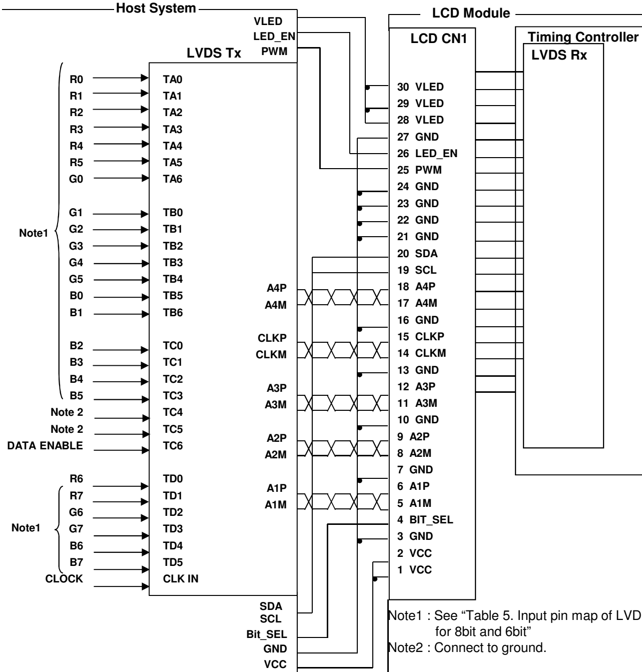
Fig 1. REQUIRED SIGNAL ASSIGNMENT FOR LVDS TRANSMITTER(THC63LVDM83R) – 8Bit
