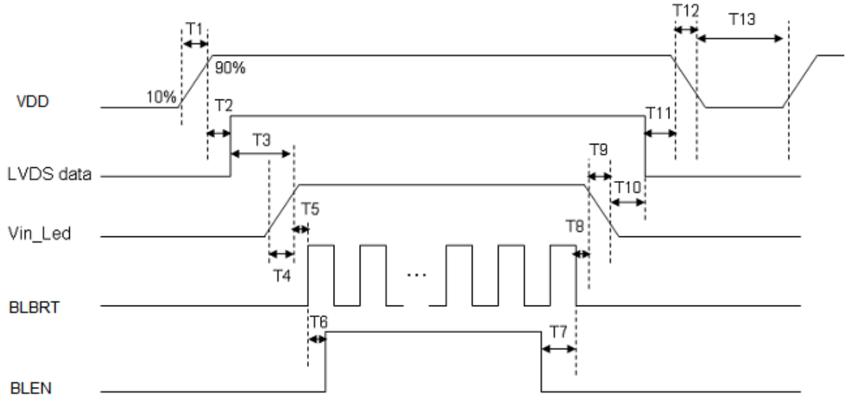
Figure 9-3 Power Sequence
