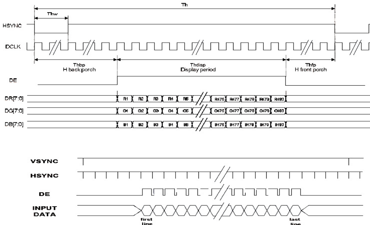
Figure 8- 2 Sync-DE mode Input setup timing
