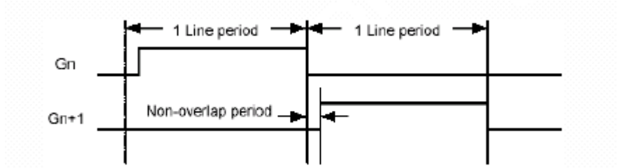
Figure 9 NO timing diagram
