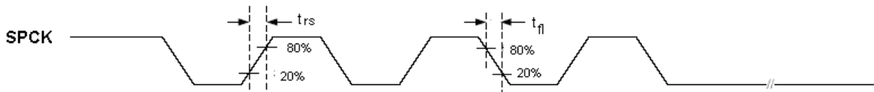
Figure 4 Rising/Falling time
