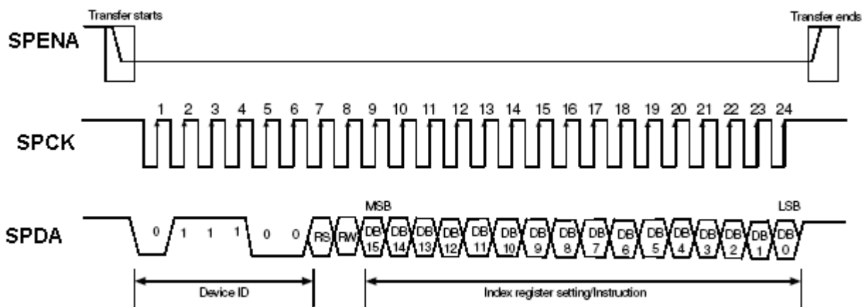
Figure 1 SPI Timing
