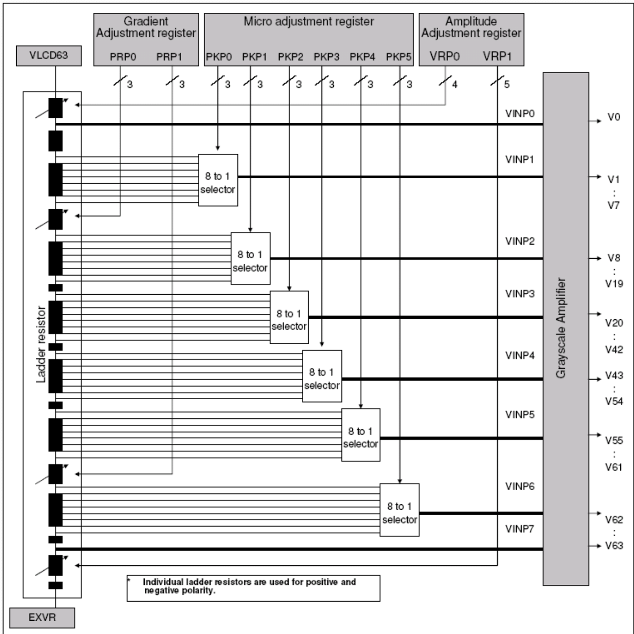
Figure 1 Grayscale amplifier
