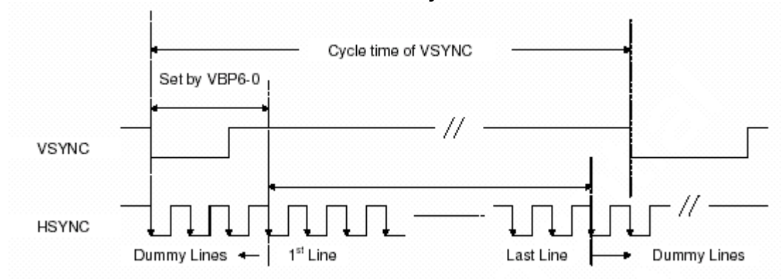
Figure 16 No. of clock cycle of HSYNC
