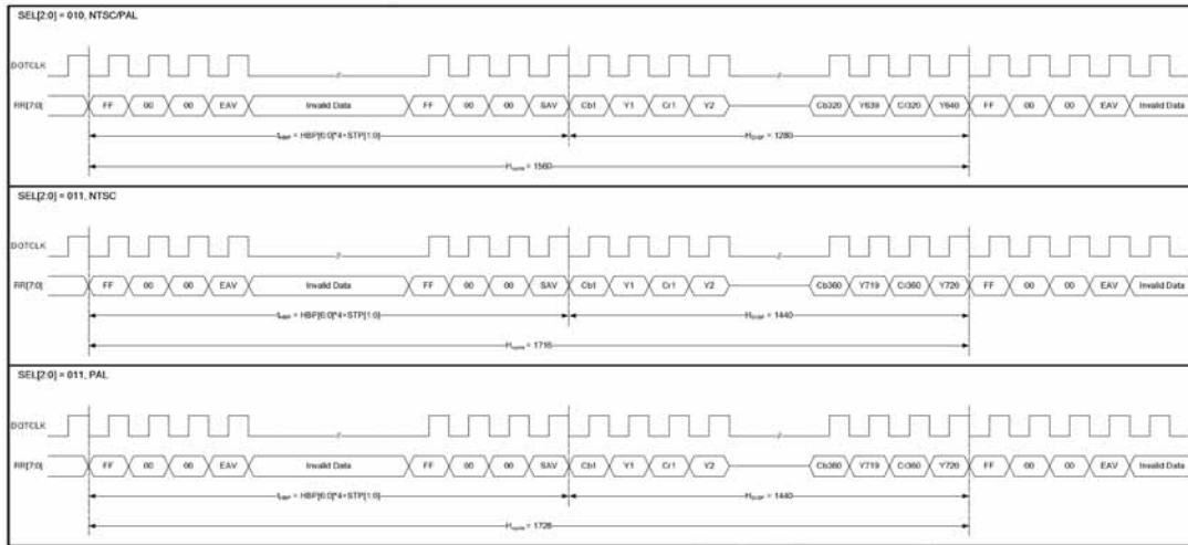
Figure 6 CCIR656 horizontal timing
