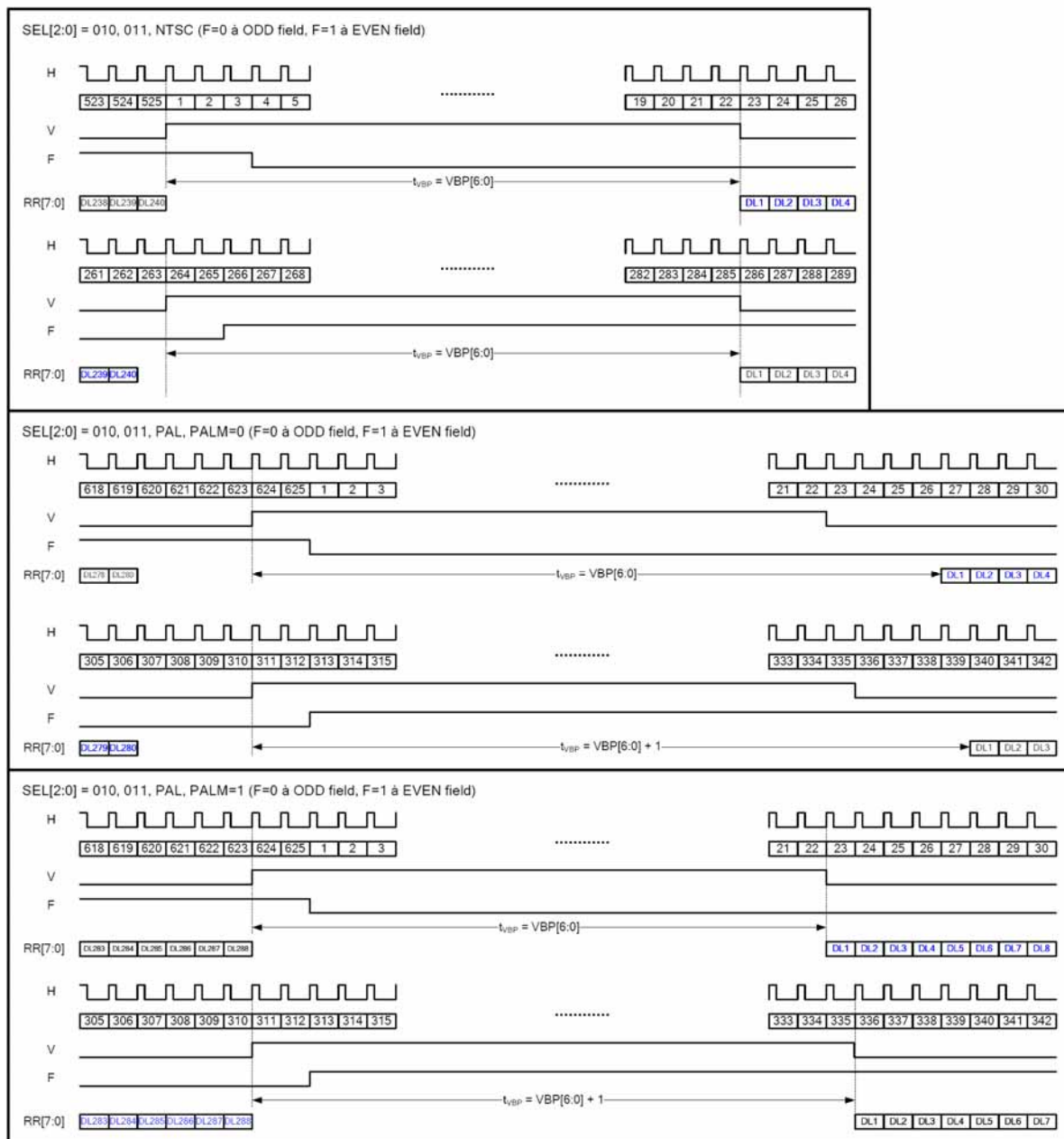
Figure 7 CCIR656 vertical timing
