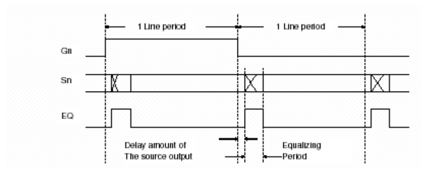
Figure 10 EQ timing diagram
