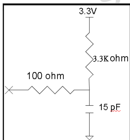
Input equivalent impedance of SDA/SCL pin
