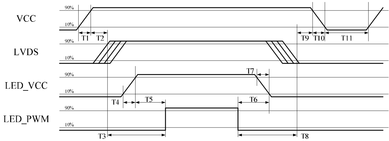
Power ON/OFF sequence timing
