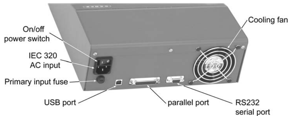
Figure 3: Rear panel of Cadex battery analyzer
