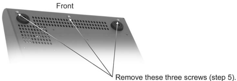
Figure 14: C7200: Remove the bottom screws
